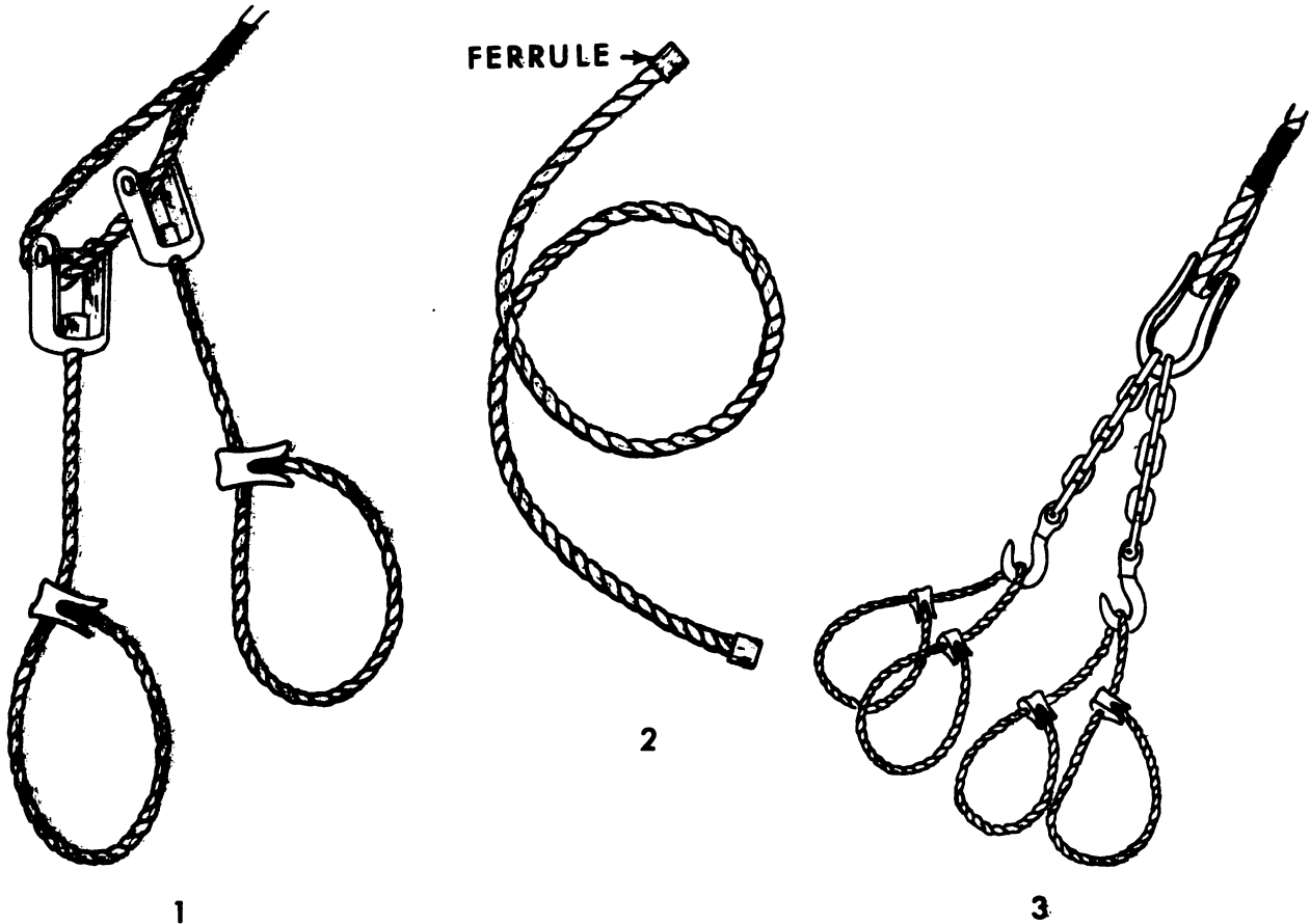
Figure 7-3. Choker hook rigging.
